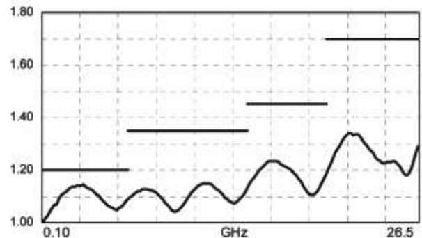
Typical V.S.W.R.
