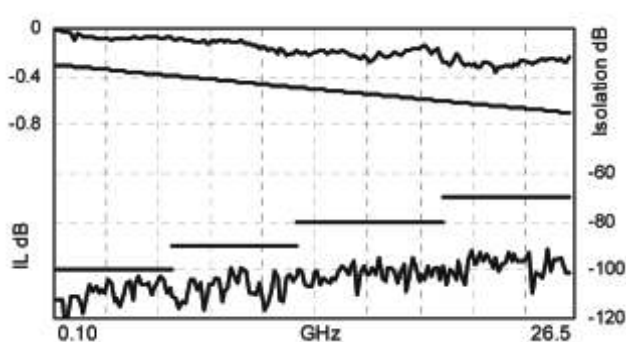
Typical ISOLATION and INSERTION LOSS
